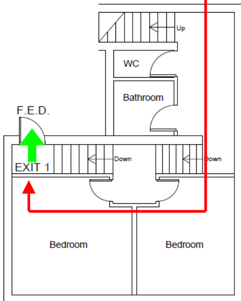
Lower Floor level (Entrance Level)
