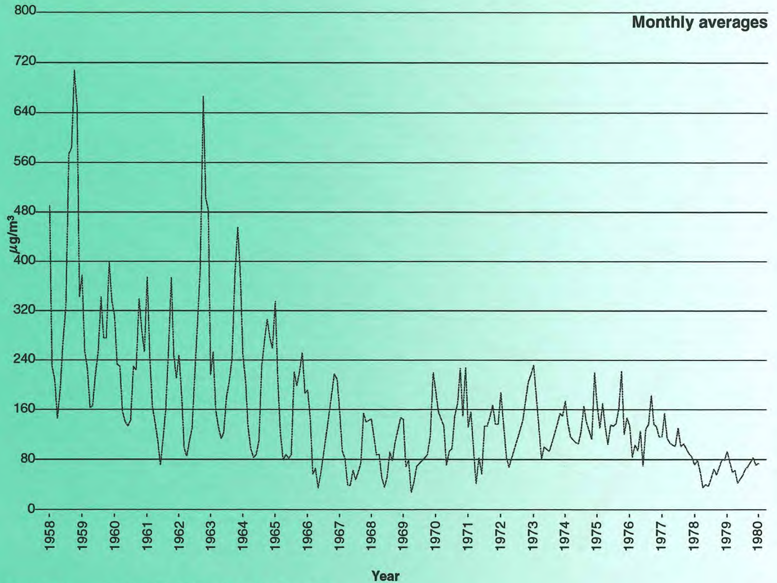
Figure 2.4 Sulphur dioxide levels at Spa Road TH April 1958 to April 1980
