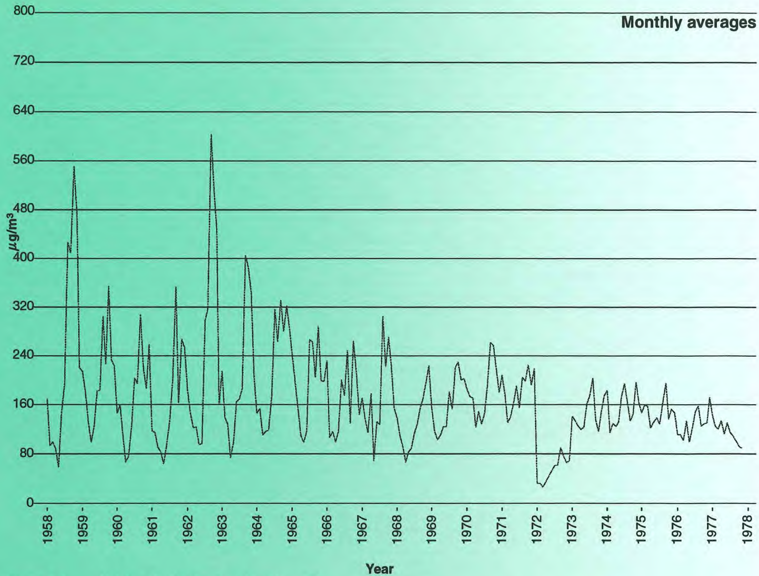
Figure 2.6 Sulphur dioxide levels at Peckham TH April 1958 to February 1978
