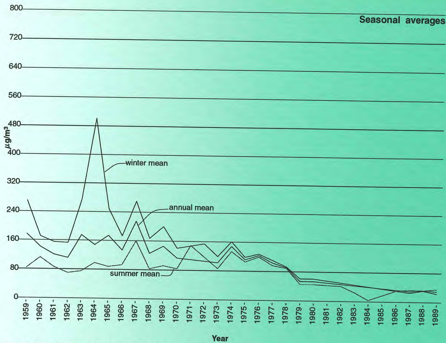
Figure 2.9 Sulphur dioxide levels at Lordship Lane 1959 to 1989
