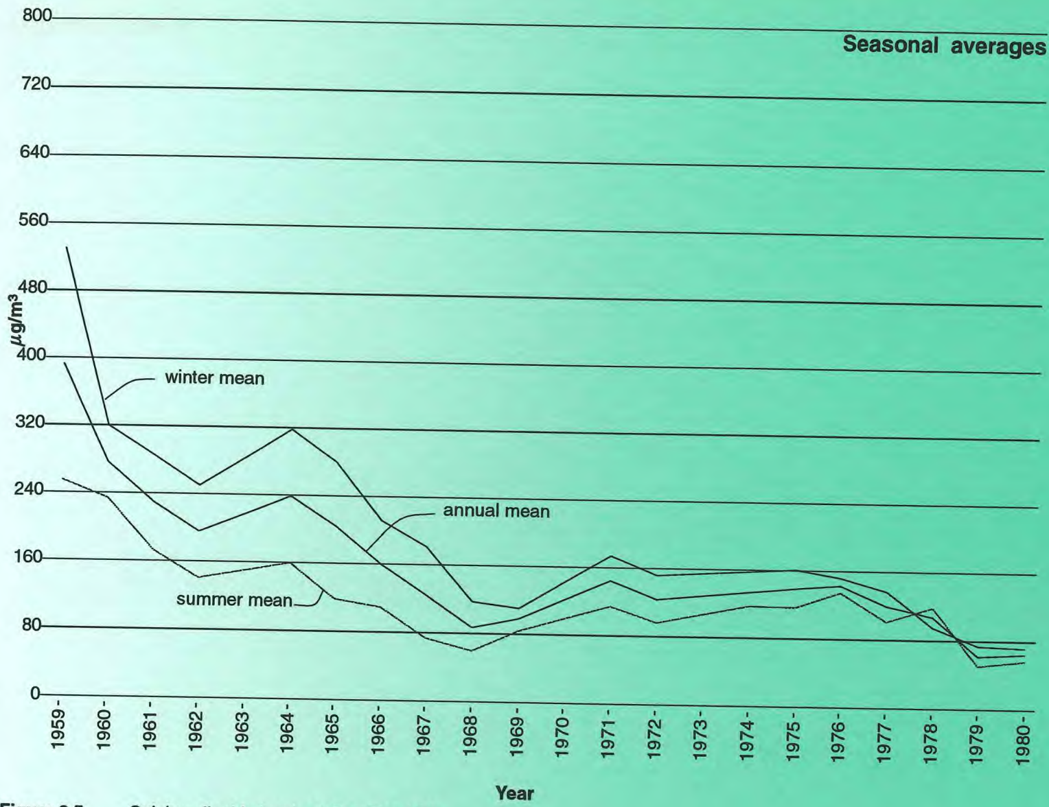
Figure 2.5 Sulphur dioxide levels at Spa Road TH 1959 to 1980
