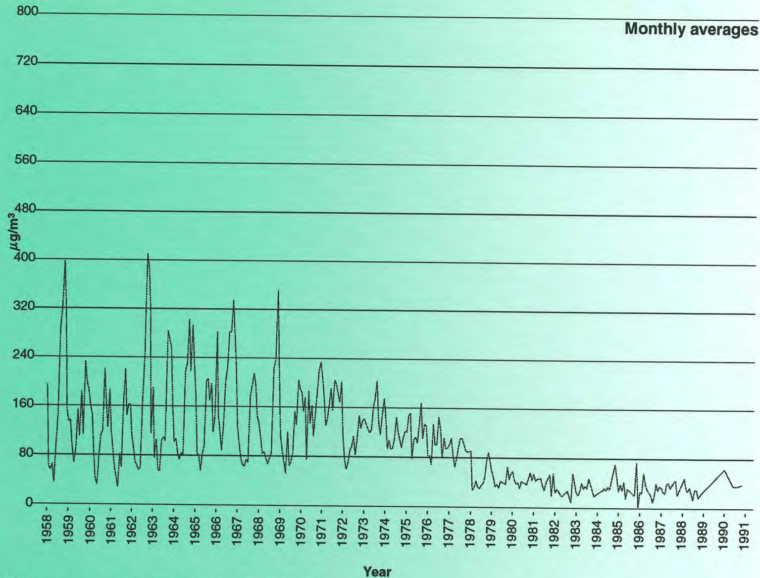
Figure 2.8 Sulphur dioxide levels at Lordship Lane April 1958 to February 1991
