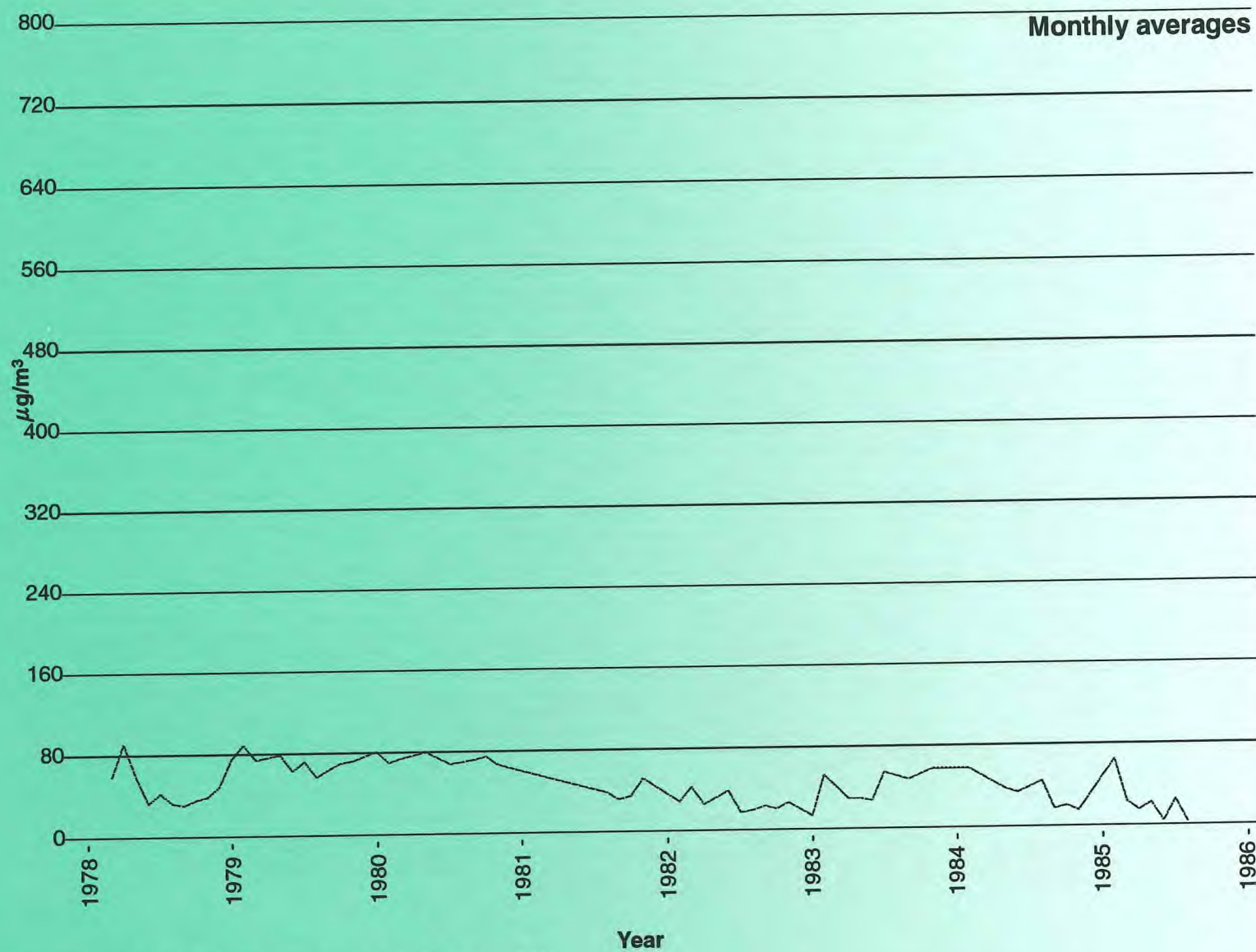
Figure 2.10 Sulphur dioxide levels at Peckham TH March 1978 to August 1985
