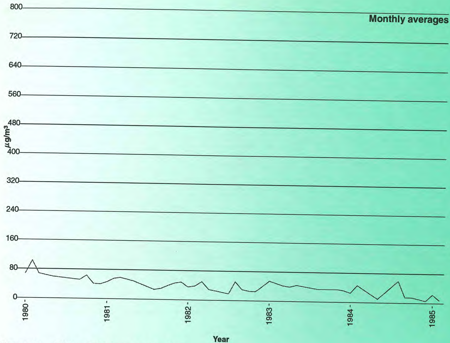
Figure 2.11 Sulphur dioxide levels at Keyse Road July 1980 to August 1985
