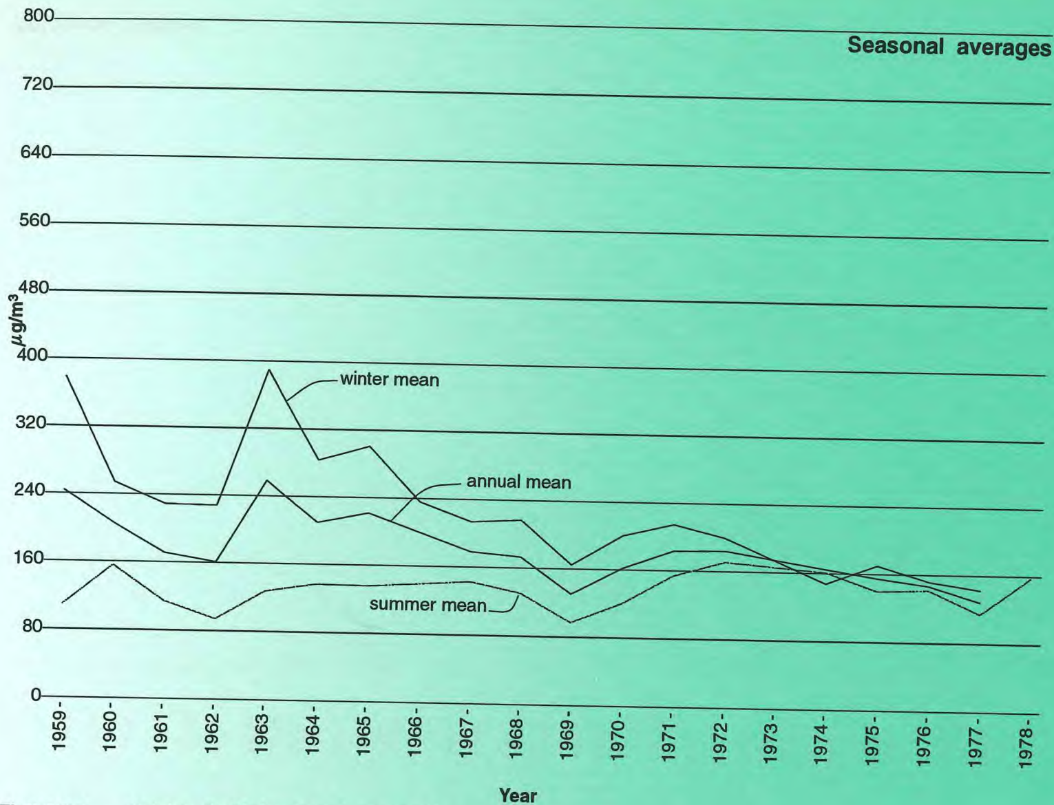
Figure 2.7 Sulphur dioxide levels at Peckham TH 1959 to 1978
