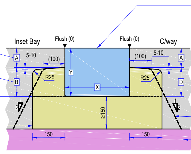
D5a - Interface with carriageway (type 0 profile kerb - general purpose)
