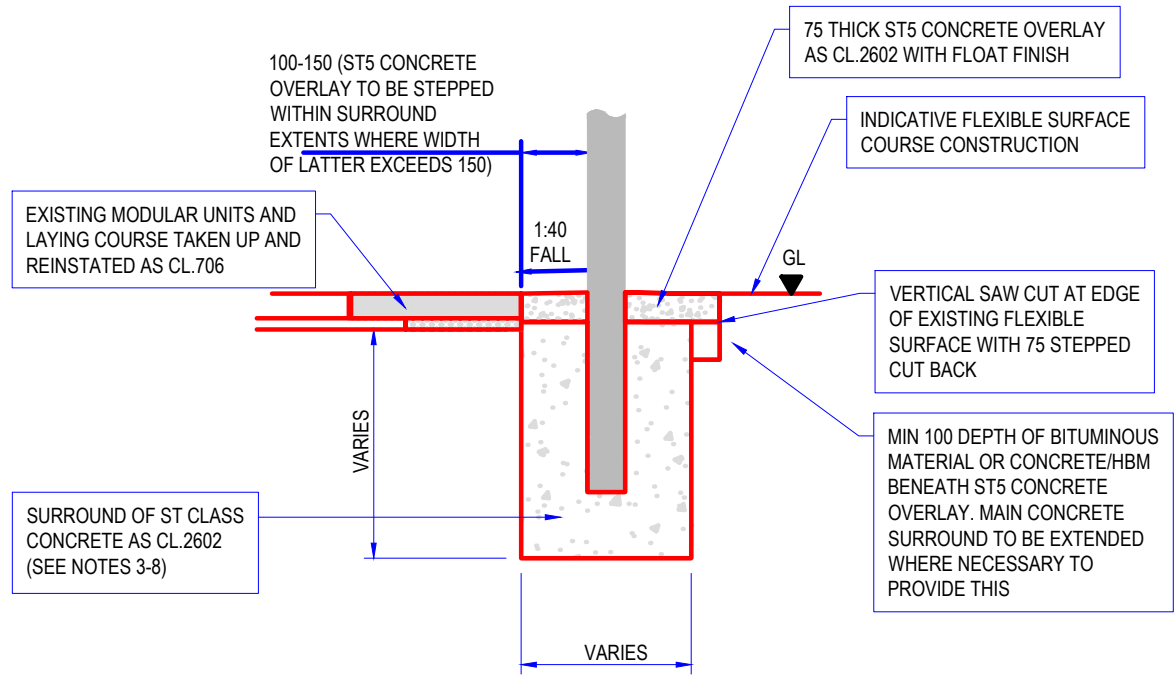
TYPE F - SECTION
