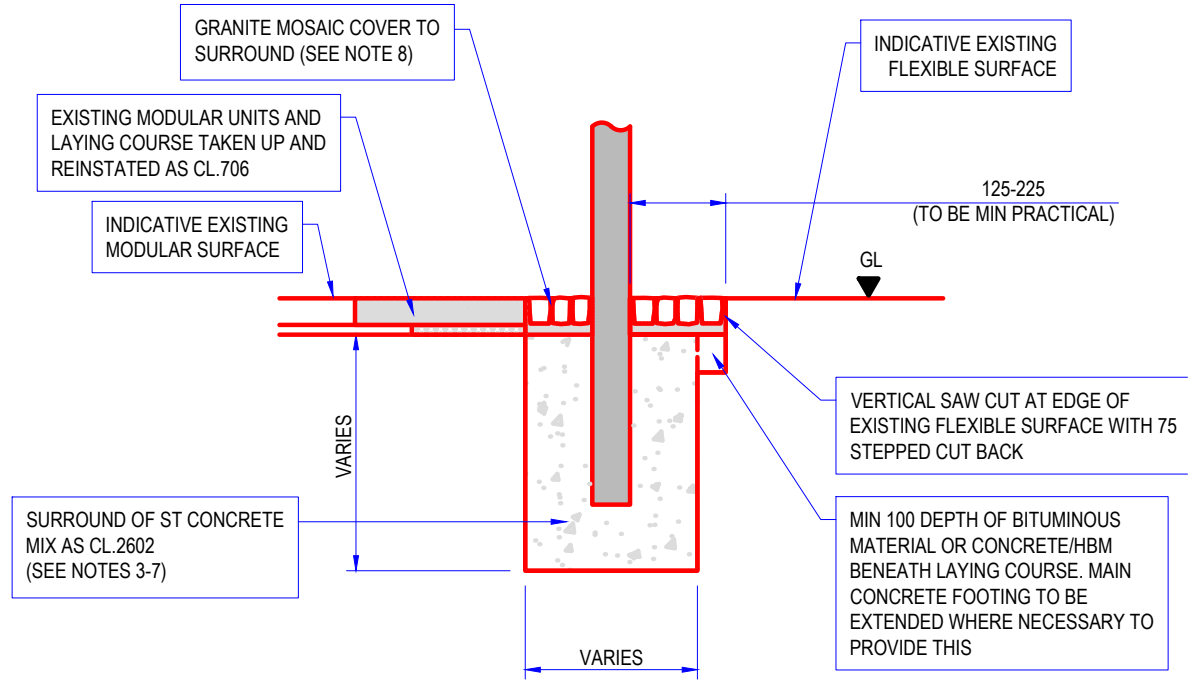
TYPE E - SECTION
