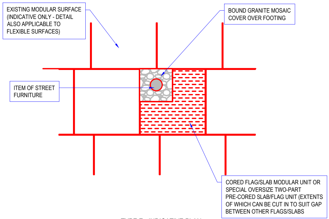
TYPE E - INDICATIVE PLAN
