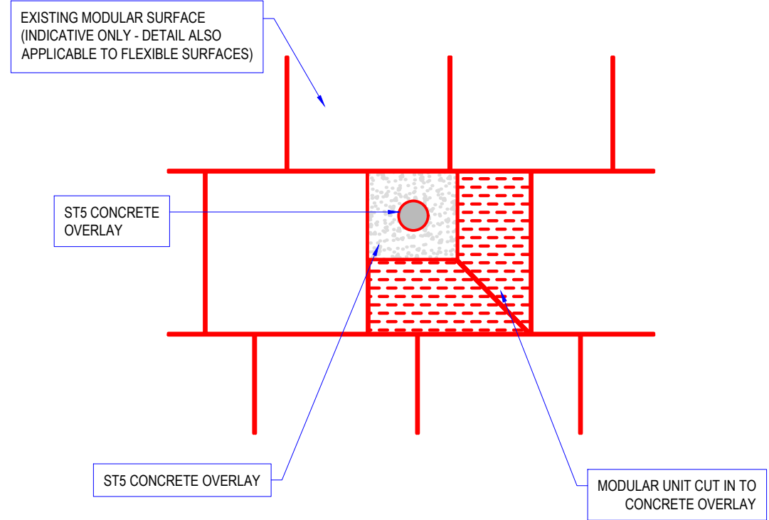
TYPE F - INDICATIVE PLAN
