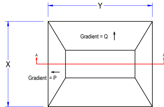
SPEED CUSHION - PLAN SCALE - 1:10
